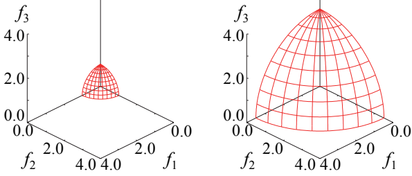
(a) Original three-objective DTLZ2. (b) Maximization version of DTLZ2. Fig. 9. Pareto fronts of three-objective DTLZ2 and Max-DTLZ2 problems.
