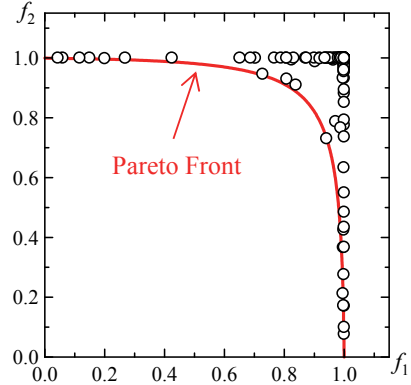
Fig. 1. Randomly generated 200 solutions and the Pareto front of a test problem in Fonseca & Fleming [2].
