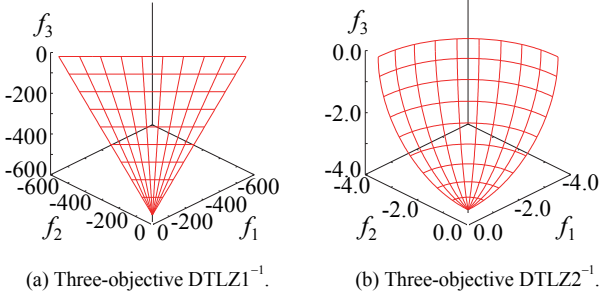
(a) Three-objective DTLZ1^{-1} . (b) Three-objective DTLZ2^{-1} . Fig. 10. Pareto fronts of the minus versions of DTLZ1 and DTLZ2.
