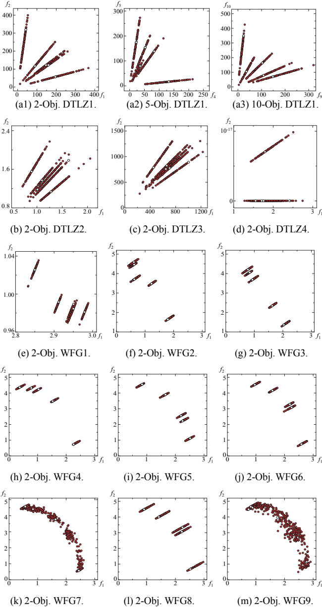
Fig. 18. Generated solutions by changing distance variables.
