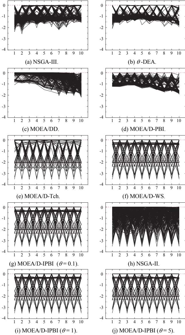
Fig. 15. Experimental results on the ten-objective DTLZ2 -1 test problem.
