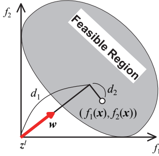
Fig. 7. Search for a solution using the weight vector w in MOEA/D.
