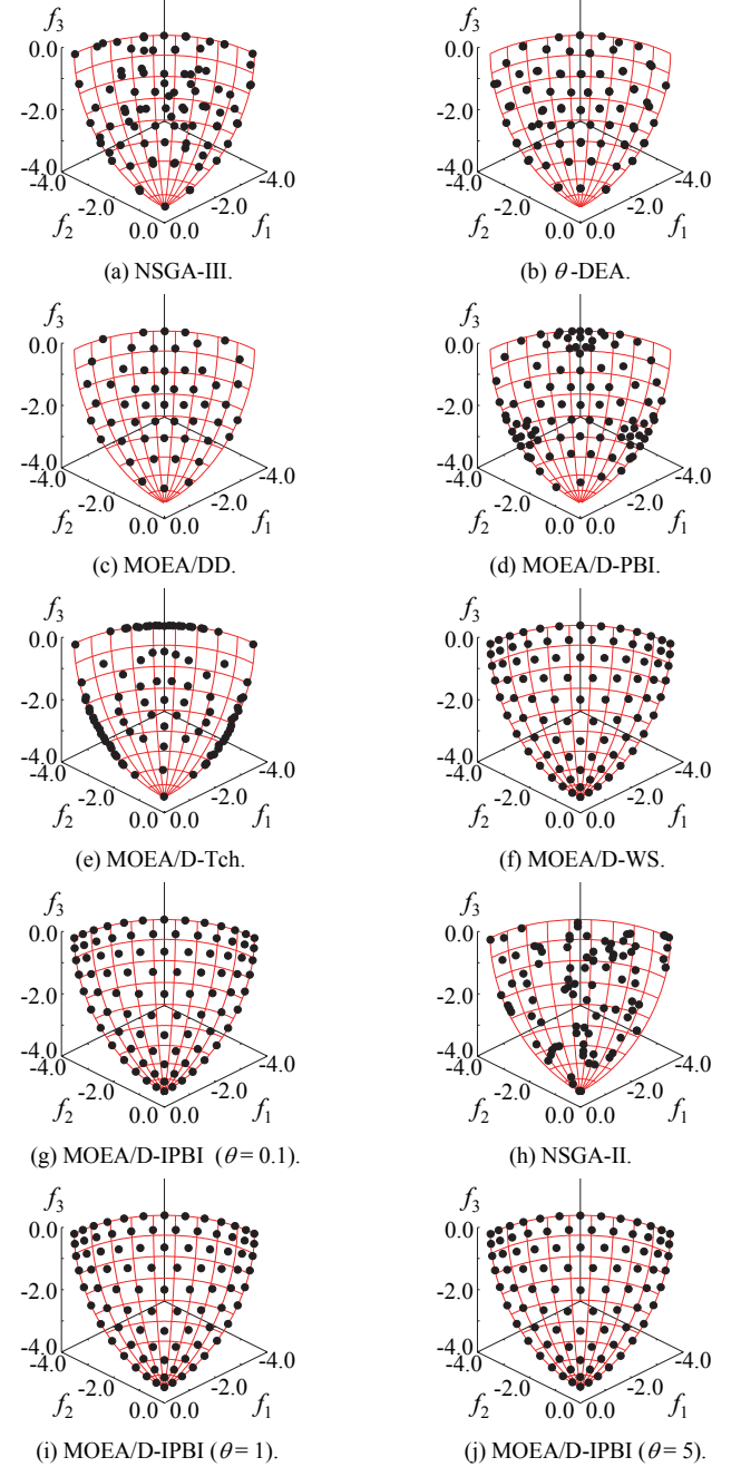
Fig. 14. Experimental results on the three-objective DTLZ2 -1 test problem.
