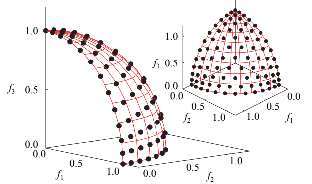
Fig. 4. Example of obtained non-dominated solutions by MOEA/D-PBI for a three-objective DTLZ2 problem using the 91 weight vectors in Fig. 3.
