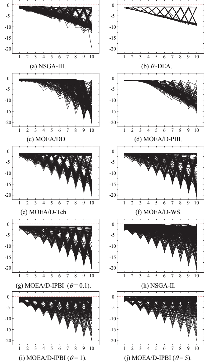
Fig. 16. Experimental results on the ten-objective WFG9 -1 test problem.
