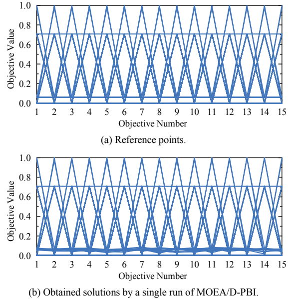
Fig. 5. Reference points for the IGD calculation and a set of obtained solutions by MOEA/D-PBI with \theta = 5 for a 15-objective DTLZ2 problem.
