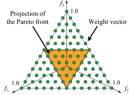
Fig. 12. Relation between a set of weight vectors and the Pareto front.
