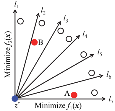
Fig. 8. Illustration of reference lines and generated solutions A and B.
