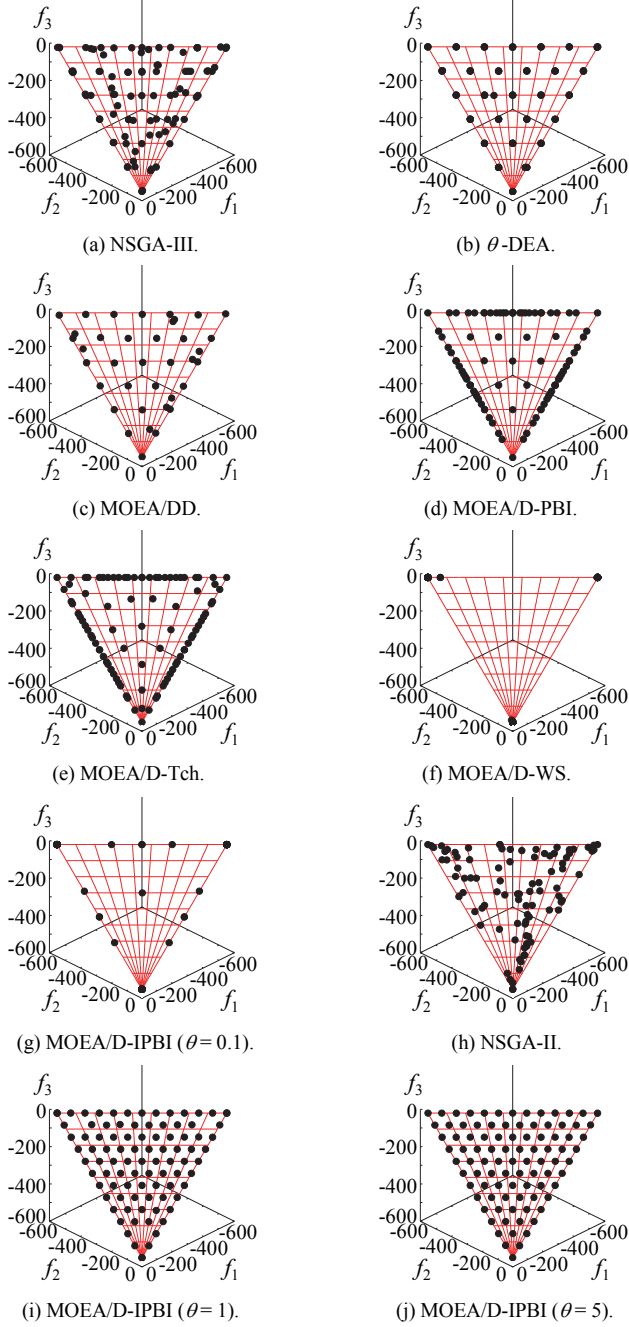
Fig. 11. Experimental results of a single run of each algorithm on the three-objective DTLZ1 -1 problem.
