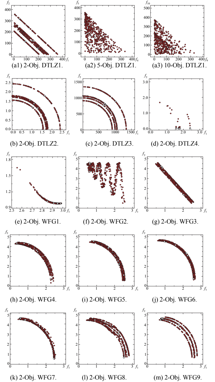
Fig. 19. Generated solutions by changing position variables.
