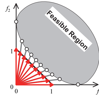
Fig. 6. Basic idea of MOEA/D and weight vector-based algorithms.
