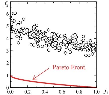
Fig. 2. Randomly generated 200 solutions and the Pareto front of a two-objective ZDT1 problem [5].
