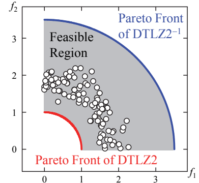
Fig. 17. Pareto fronts of the two-objective DTLZ2 and its maximization version Max-DTLZ2 which is equivalent to the two-objective DTLZ2 -1 .
